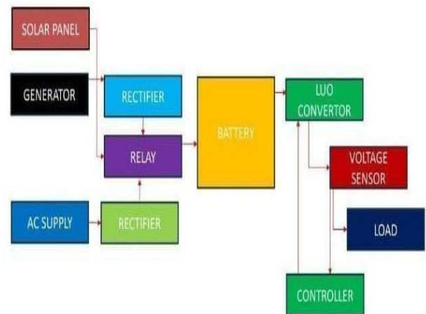
Figure 1 Block Diagram of Battery Working System in LUO Converter to Load
