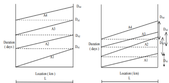
Figure 4 Network Diagram Duration Plot as per CPM Distance –Duration Plot as per LSM
