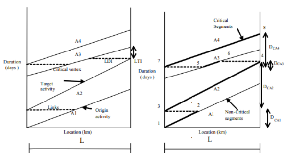
Figure 5 Activity Sequence Downward Pass Upward Pass
