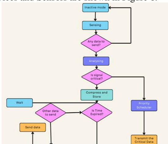
Figure 6 Real-Time Activities Monitoring Wearable Devices and Sensors
