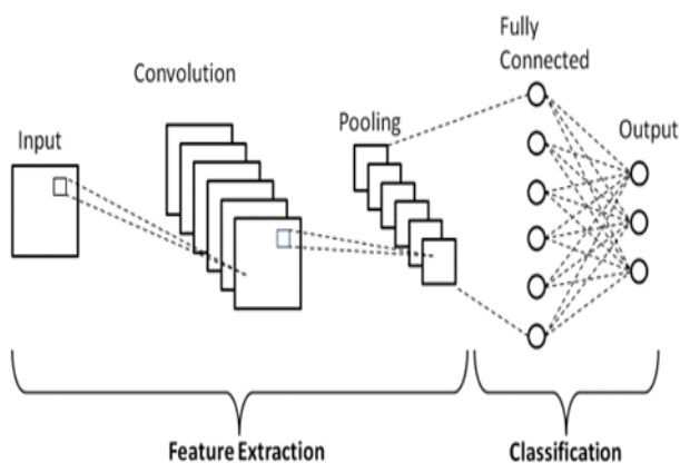
Figure 2 CNN Architecture
