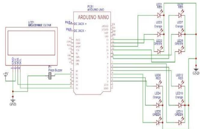
Figure 4 Coordination of LED Lights with Arduino Nano
