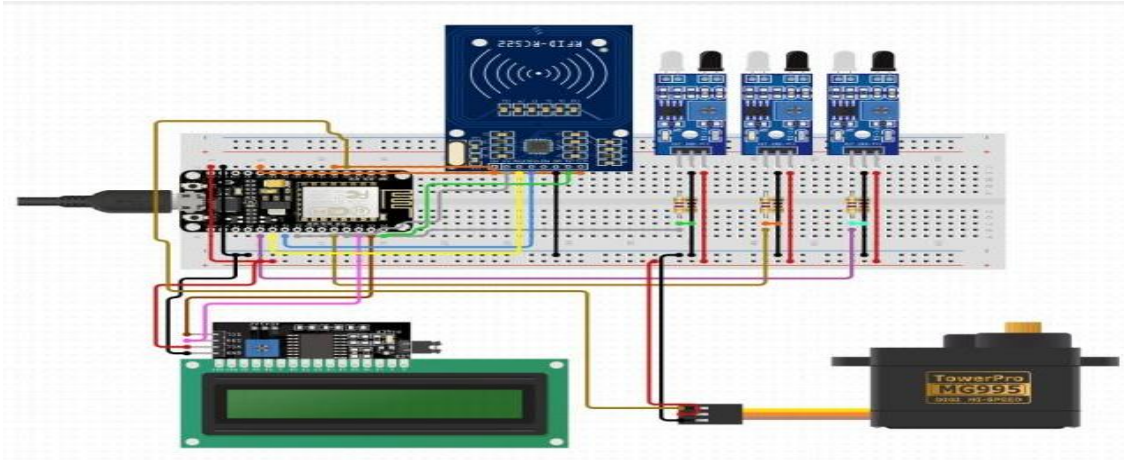
Figure 2 Circuit Diagram
