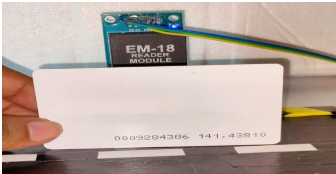
Figure 12 RFID Tag Kept Near the Scanner
