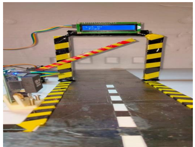
Figure 5 RFID scanner, LCD Display, Servo Motor at the gate
