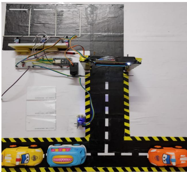
Figure 3 Overall Setup
